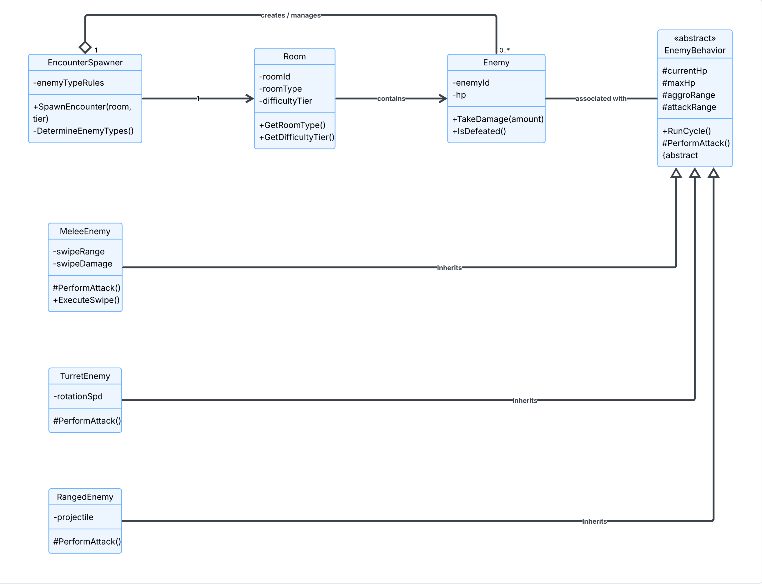
Enemy Encounter Class Diagram
